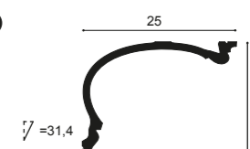
C343 HERITAGE A 200 x 19 x 25 cm Purotouch ®
